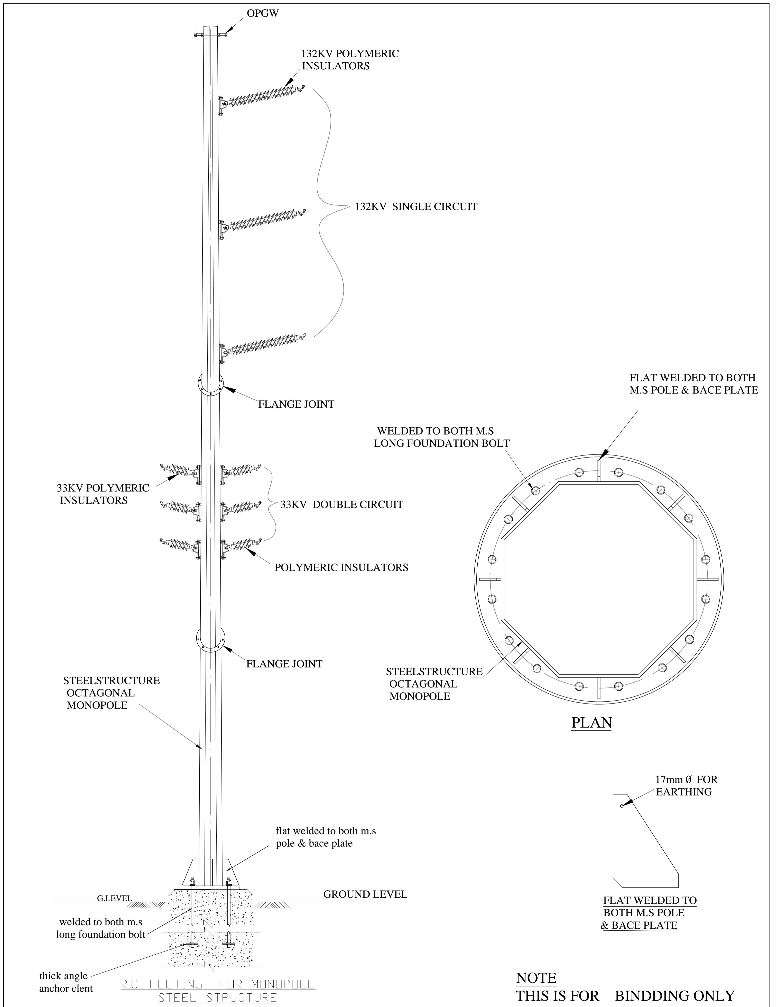
TYPICAL DRAWING OF PROPOSED OCTAGONAL MONOPOLE ( 132KV SELF SUPPORTING TOWER)
